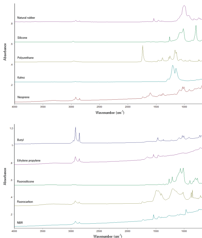
Figure 4 and 5. Spectra of seals were recorded using a 20 second co-addition of interferograms at 8\text{ cm}^{-1} resolution. The spectra are offset for clarity.
